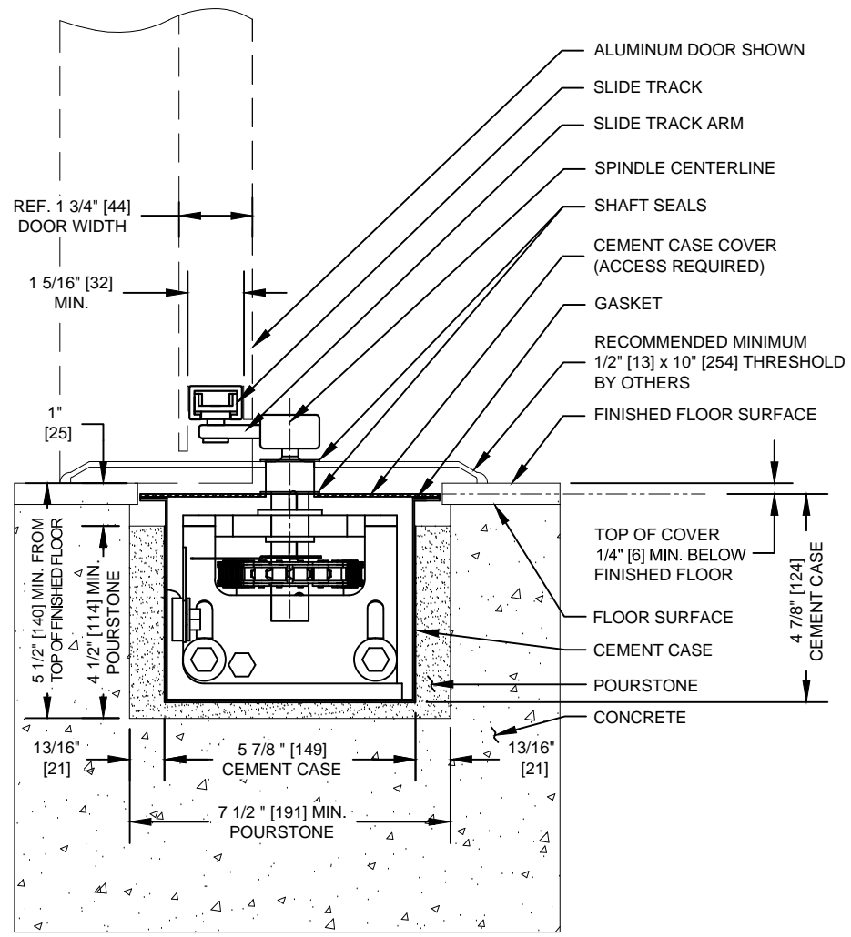
SECTION 2 ED250-IG SLIDE TRACK OPERATOR
