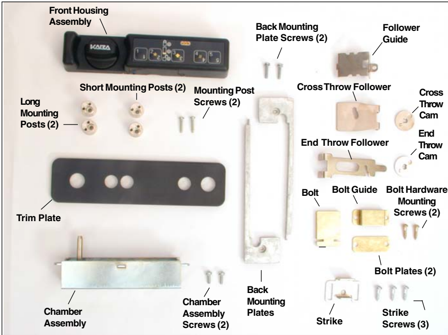
Figure 1 - Unicon CL20 Wood Dead Bolt Lock Parts
