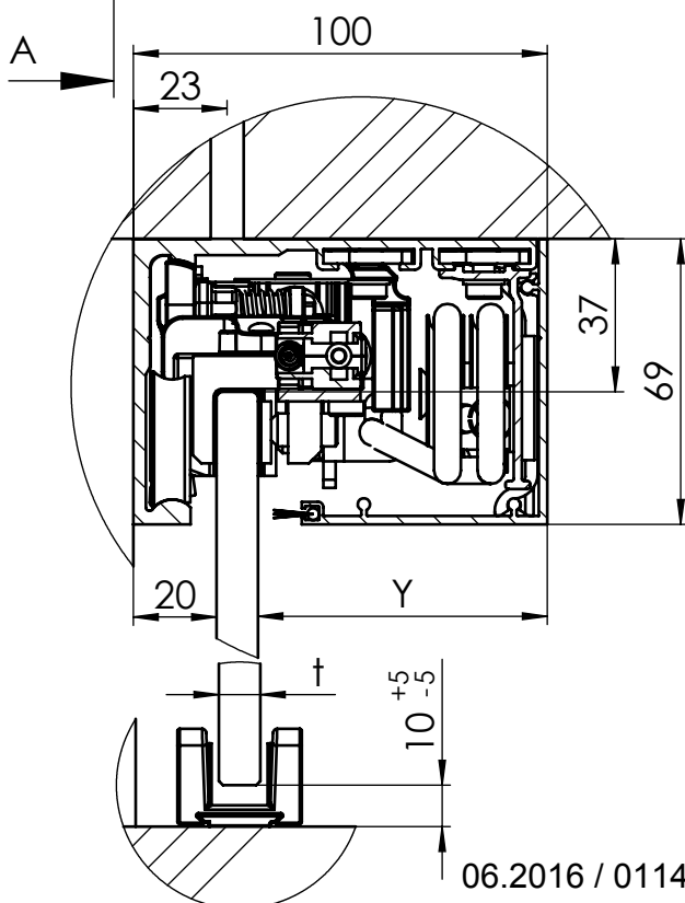
Detail X (1 : 2)
