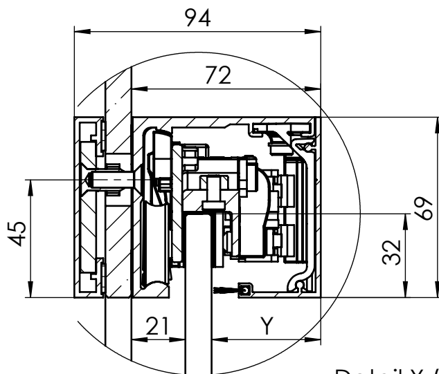
Detail X (1 : 2)
