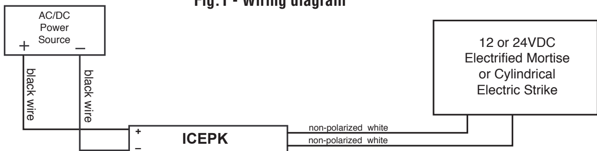
Fig.1 - Wiring diagram
