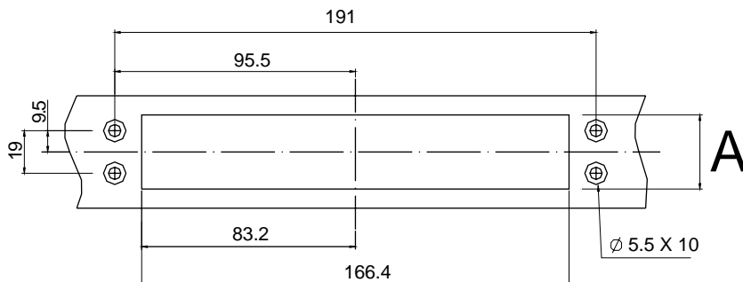
Mounting on metallic door
