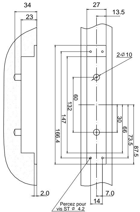
Typical installation for wooden door (GB)
