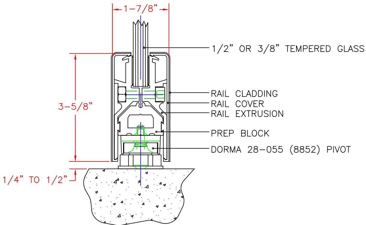
SECTION THRU DOOR AND RTS CLOSER
