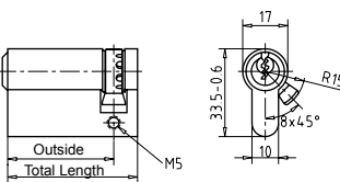
Security single cylinders with 5 pins
