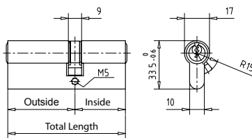
Security double cylinder with 5 pins
