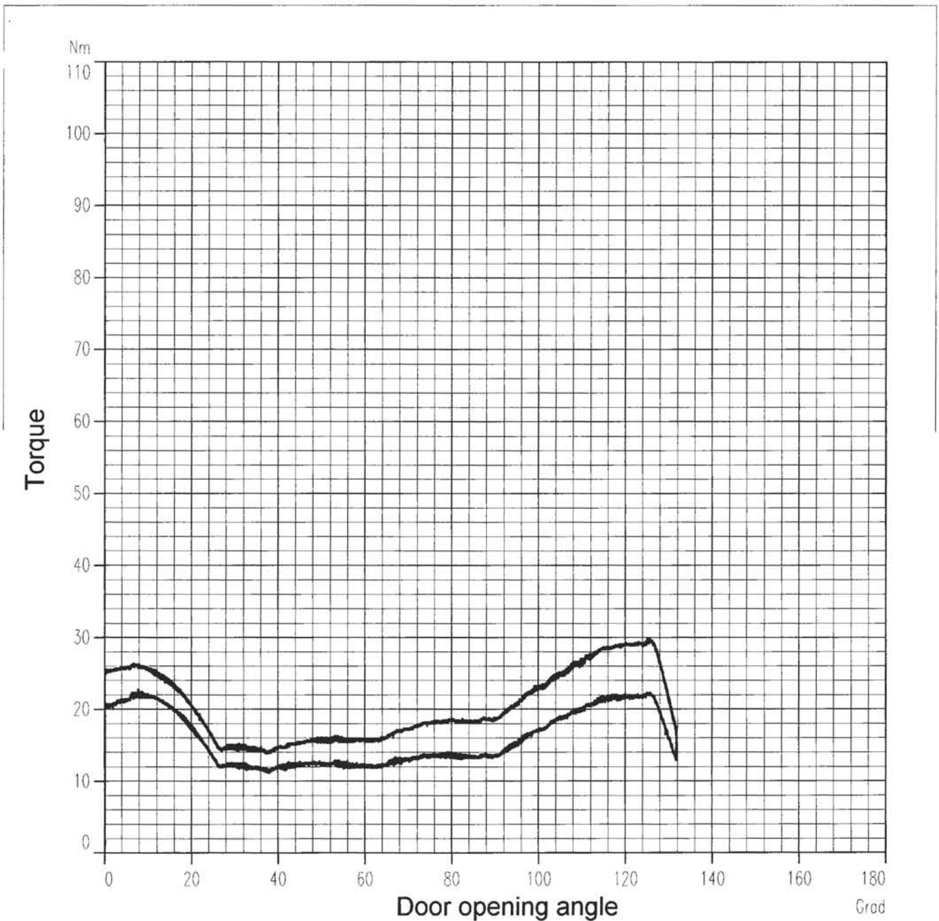
Torque curve
