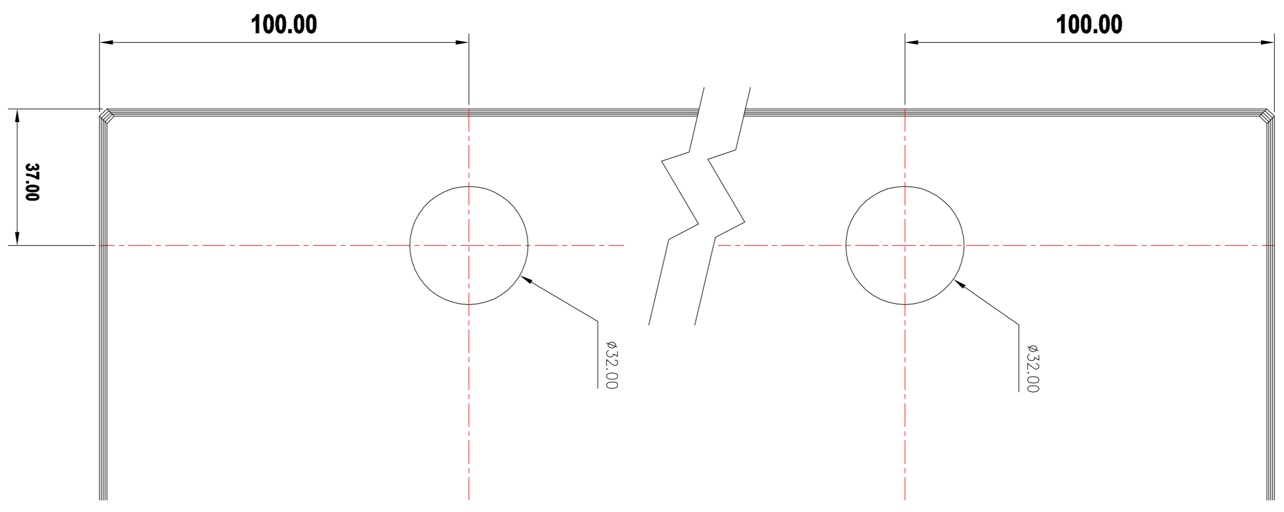
12 mm Thick Glass Door Hole Detail
