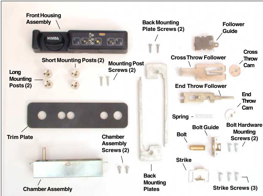
Figure 1 - Unicon CL20 Wood Spring Latch Bolt Lock Parts
