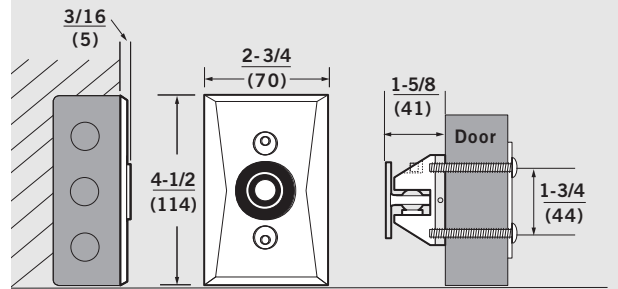
Overall Projection: 1-13/16" (46)
