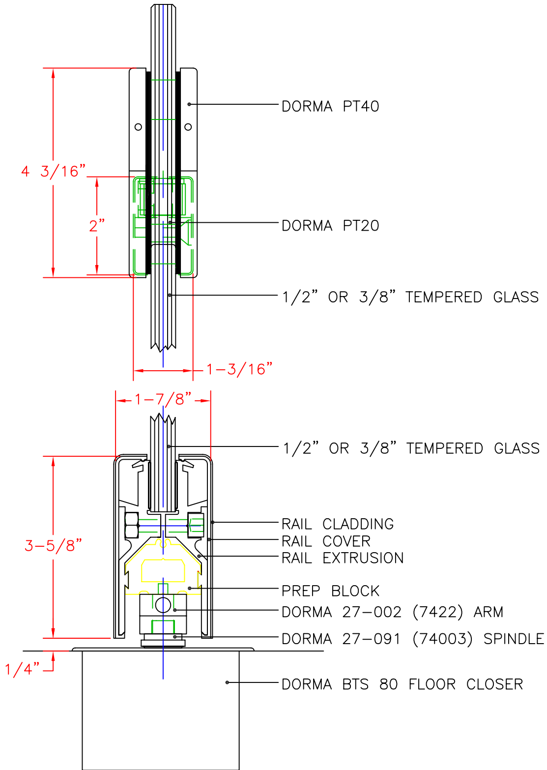
SECTION THRU DOOR AND BTS CLOSER
