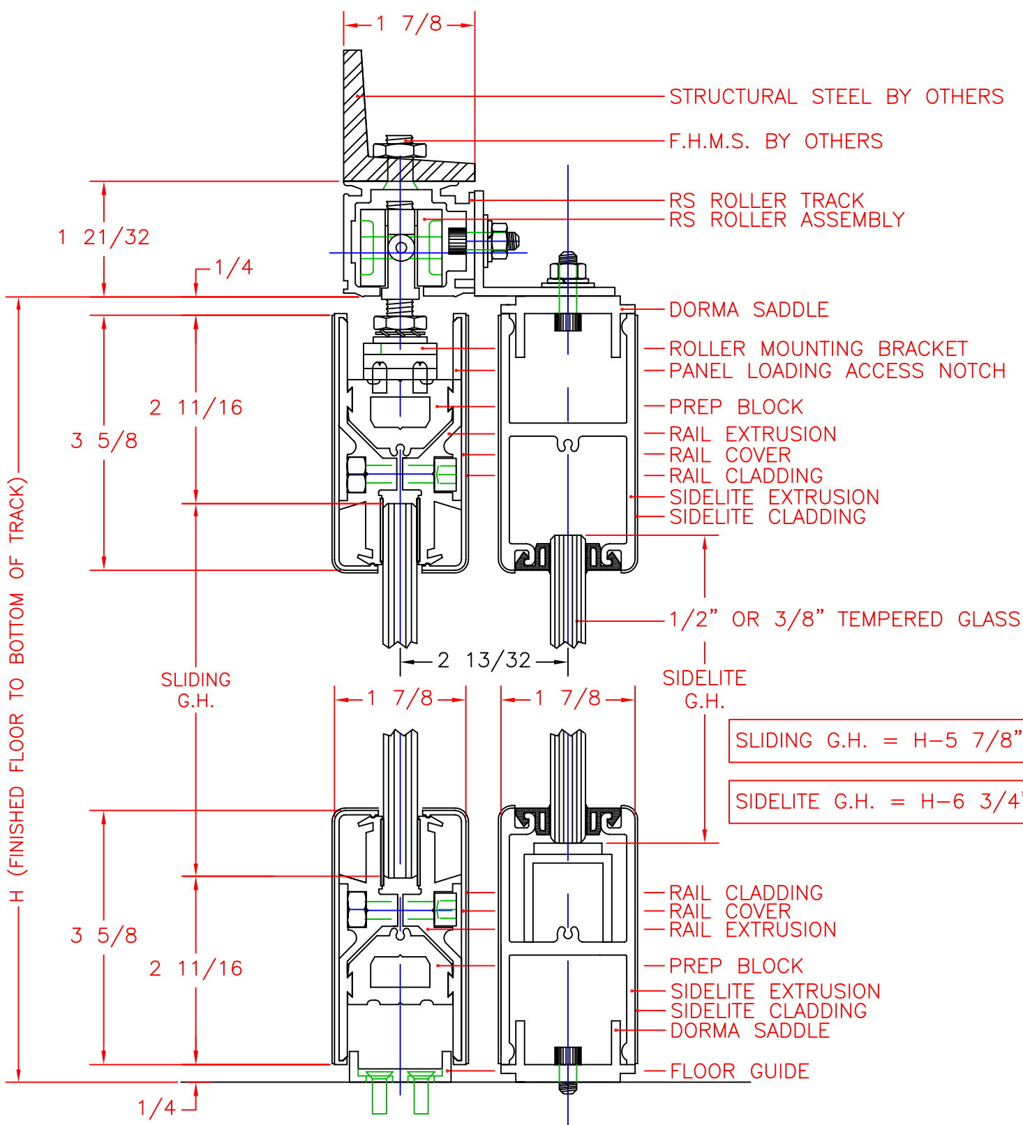
RS-DRS SECTION THRU SLIDING PANEL AND SIDELITE
