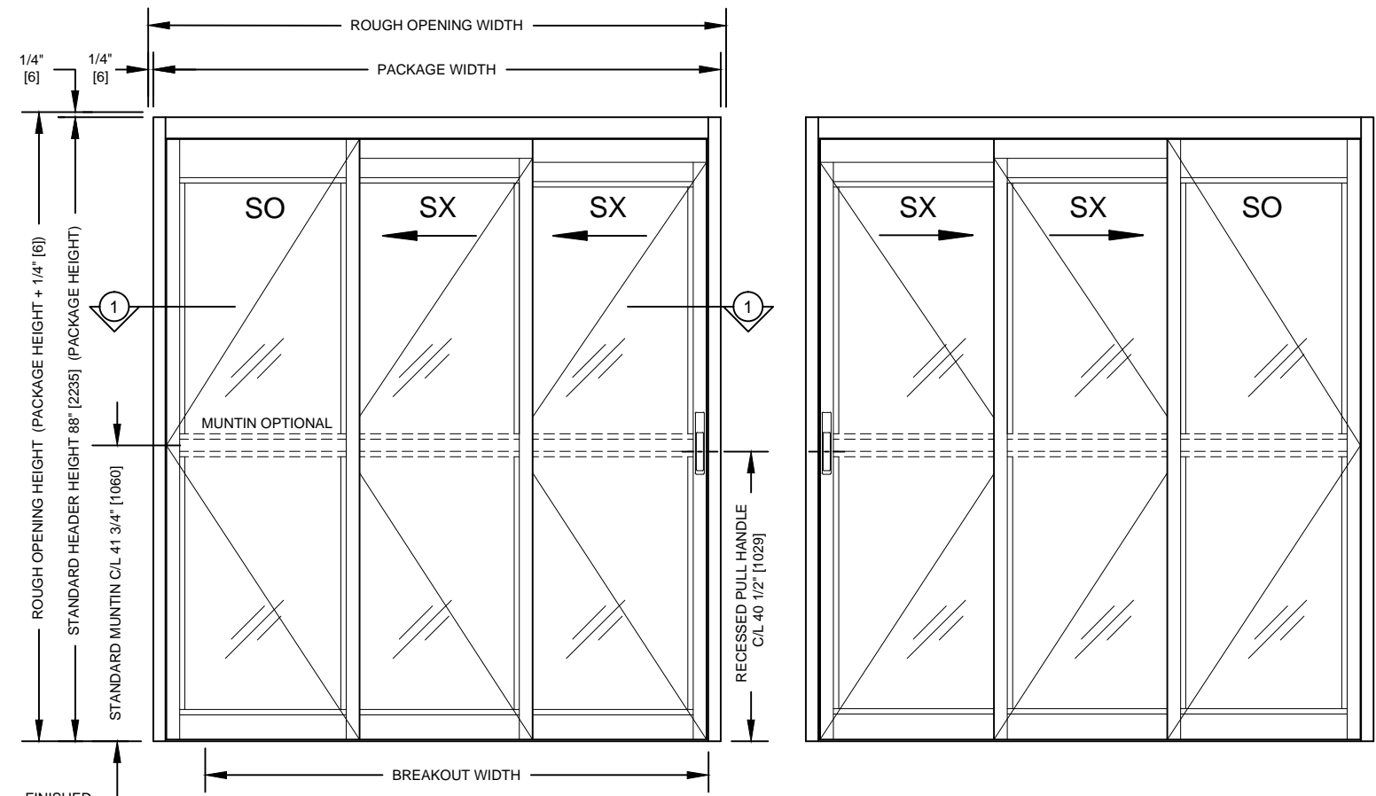
EXTERIOR ELEVATION TYPE: SO-SX-SX, SX-SX-SO
