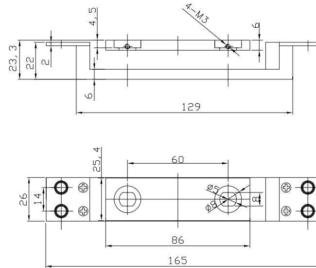
armature dimensions
