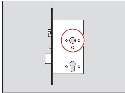
1 x 7mm Reduzierhülsen / Reducing sleeve Art.Nr.: 70930050
