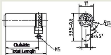
Security single cylinders with 5 pins
