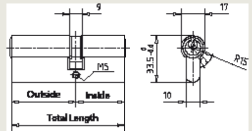
Security double cylinder with 5 pins
