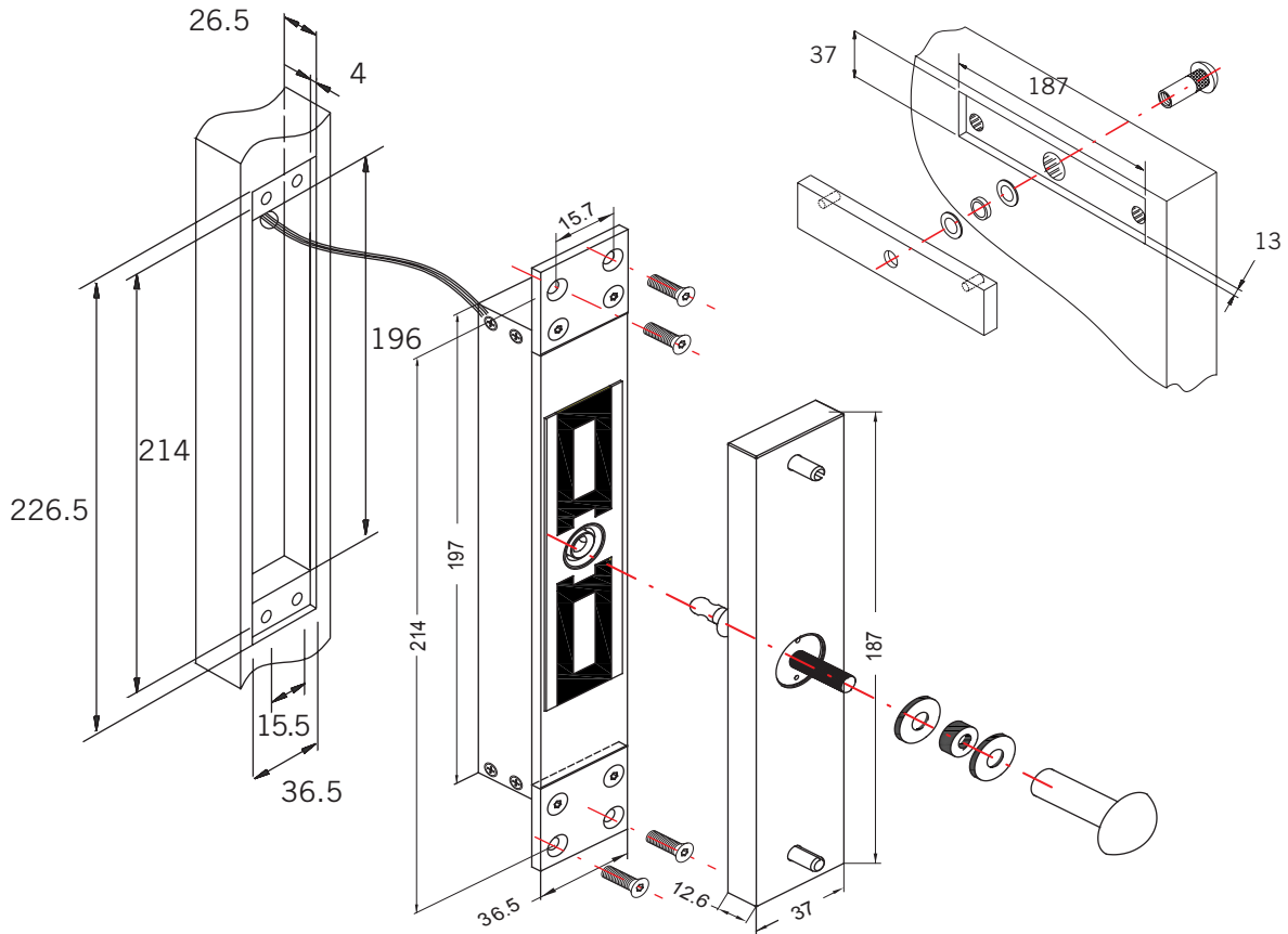
Typical installation for wooden door (GB)
