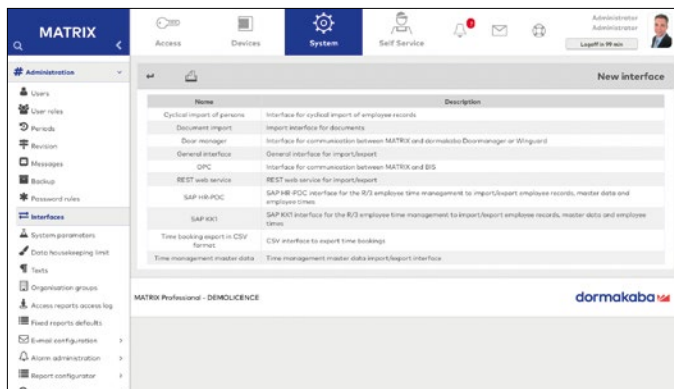
Interface selection
